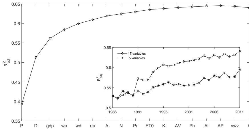
Fig. 5.7 Stepwise selection of the major drivers of the virtual water flows in year 2011 for a network of 117 nodes, by adopting the R_{adj}^2 value as the comparison criterion, using a 17-variables regression. The inset reports the temporal trend of the worldwide adjusted coefficient of determination, considering a 17-and a 5-variables regressions.
