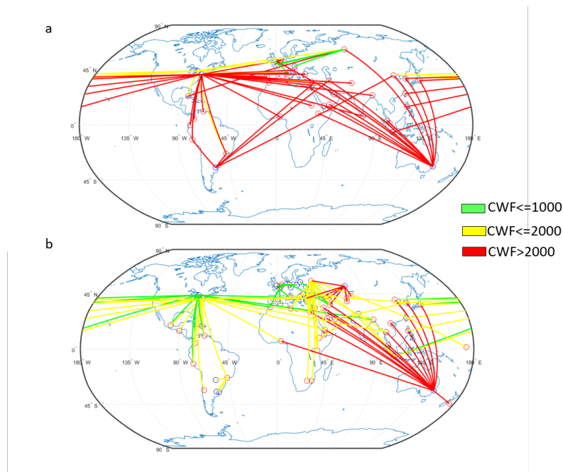
Fig. 3.6 The efficiency of virtual water trade in 1986 (a) and 2013 (b). Link color stands for the CWF of wheat in the country of export: green indicates CWF \leq 1000 \text{ m}^3 \cdot \text{ton}^{-1} , yellow indicates a CWF in the range (1000; 2000] \text{ m}^3 \cdot \text{ton}^{-1} , red indicates that the CWF is higher than 2000 \text{ m}^3 \cdot \text{ton}^{-1} . Countries are represented through nodes: blue circles stand for exporting countries, red circles signify importing countries.
