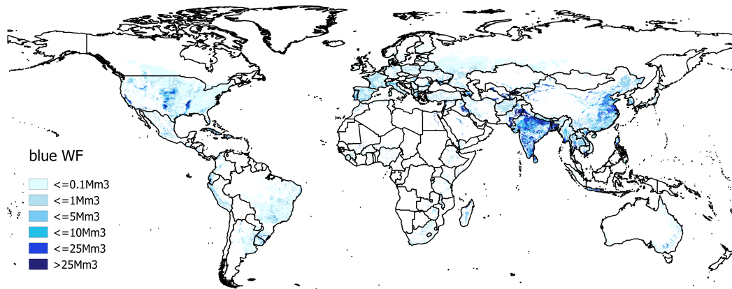
Fig. 4.5 Map of blue water footprint of crop production in year 2000.
