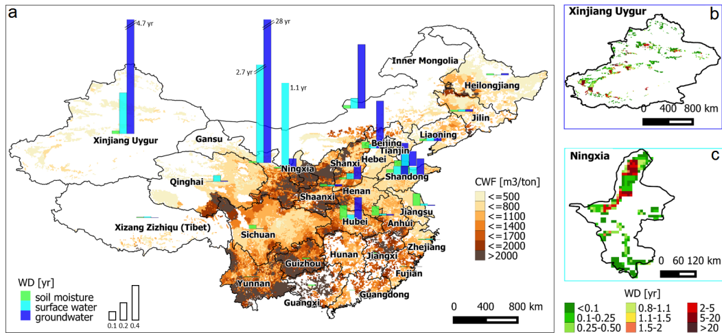
Fig. 4.9 Gridded crop water footprint (volume of water per ton of crop) of wheat in China and histograms of average water debt ( WD ) at the province level (a). Gridded groundwater debts in the Xinjiang Uygur province (b), and gridded surface water debts in the Ningxia province (c).
