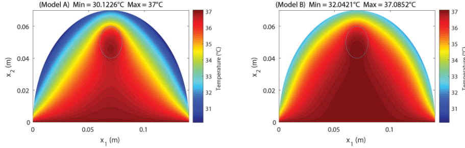
Figure 3: Temperature distribution of a cancerous breast tissue with an embedded spherical tumor of radius 1cm. The solid line represents the boundary of the heterogeneous tumor.
