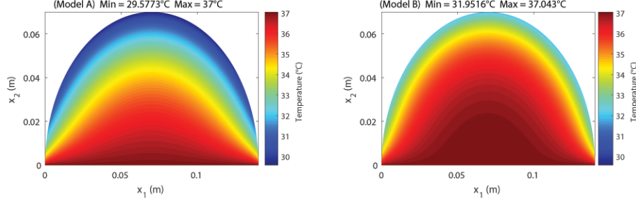
Figure 2: Temperature distribution of a healthy breast tissue.
