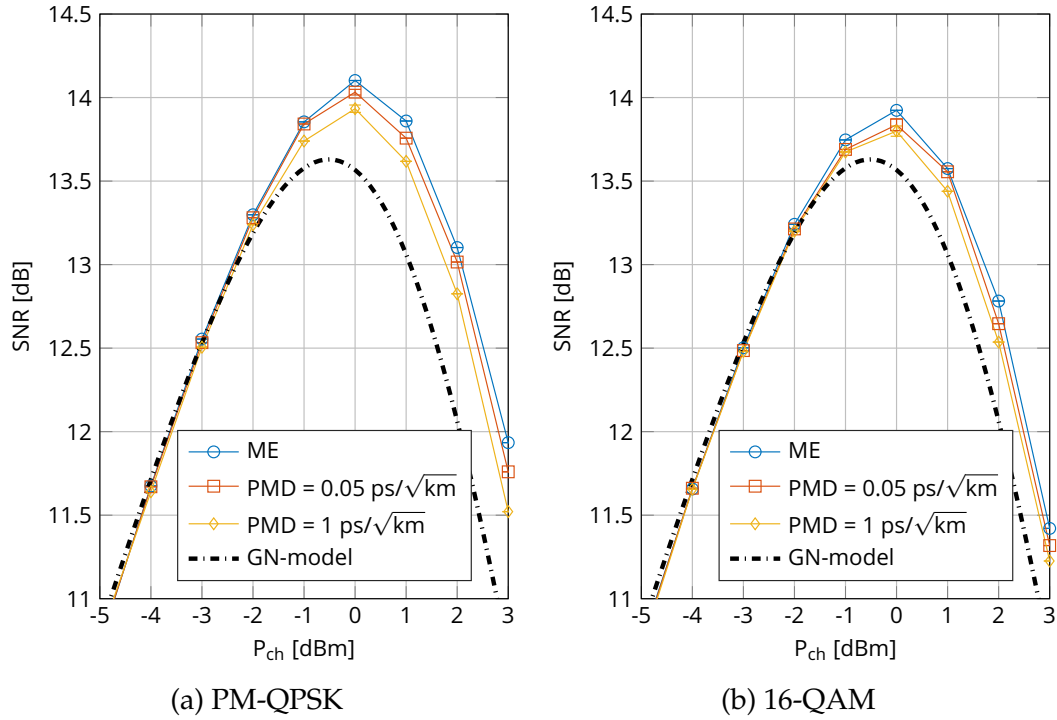
Fig. 2.6 Generalized SNR for PM-QPSK and PM-16QAM for different values of PMD in a system with 41 32-GBaud WDM channels in a 50 GHz grid, and comparison with GN-model predictions
