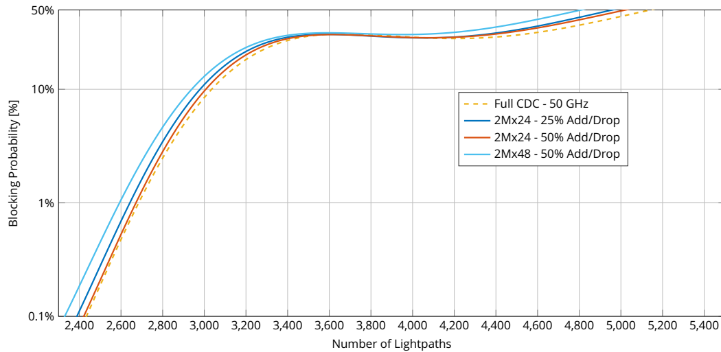
Fig. 3.25 Blocking probability vs number of allocated lighthpaths for of two different WSS architecture with different levels of add/drop capability.
