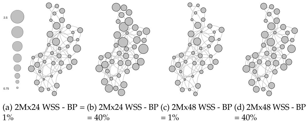
Fig. 3.24 Qualitative description of required number of WSSs per direction in each network node, for two different node configurations (2Mx24 and 2Mx48) and two different target blocking probabilities (1% and 40%). All 4 cases refer to the 50-GHz grid scenario. Node sizes varies from 0.75 to 2.5 WSS/direction.
