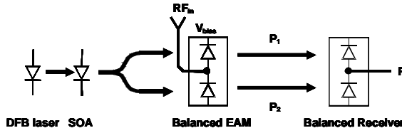
Fig. 1. Schematic of the balanced-electroabsorption-modulated link
