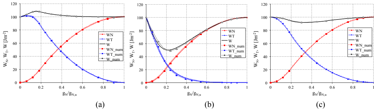
Figure 1: Work of separation for bilinear models by Högberg (a), and by Camanho et al. for a P-L criterion (b), or a B-K criterion (c). \phi_N = \phi_T = 100 N/m.
