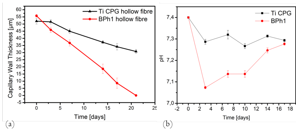
Fig. 6.7 (a) Reduction of the wall thickness of the BPh1 hollow fibre and the Ti-CPG as a function of the immersion time in PBS; (b) variation of pH in the PBS solution over time during the dissolution tests.
