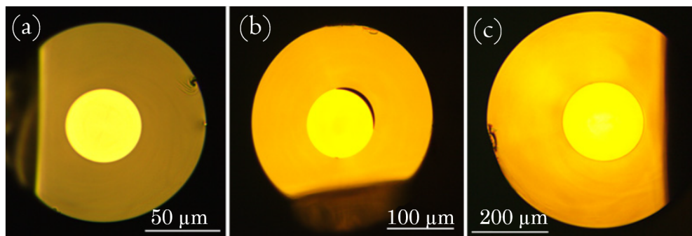
Fig. 7.2 Optical microscope pictures of multi-mode fibres and cane for TD-DOS: (a) 150 µm optical fibre; (b) 300 µm optical fibre; (c) 600 µm cane [27].
