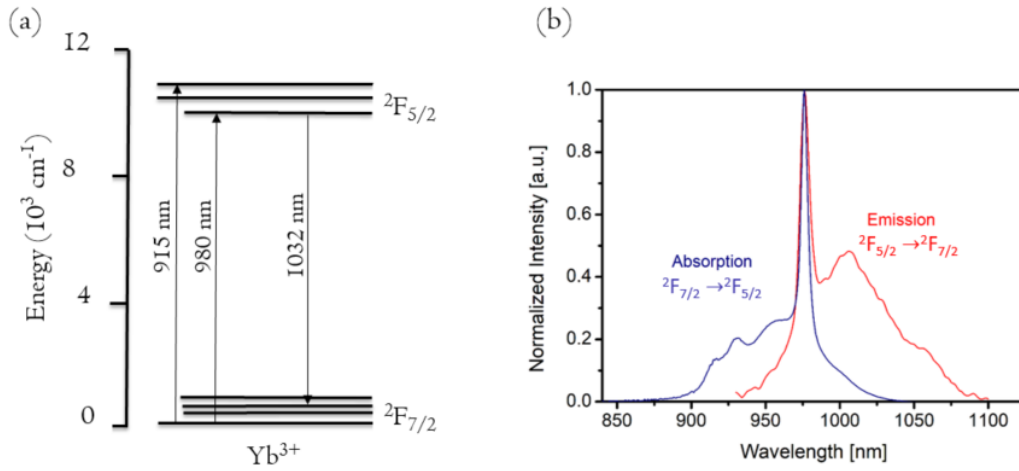
Fig. 2.5 (a) Schematic representation of the energy levels of \text{Yb}^{3+} ion (b) absorption and emission peaks related to the 2F_{7/2} \rightarrow 2F_{5/2} and 2F_{5/2} \rightarrow 2F_{7/2} transitions [7].
