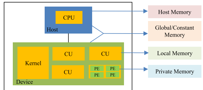
FIGURE 1. OpenCL platform and memory model.
