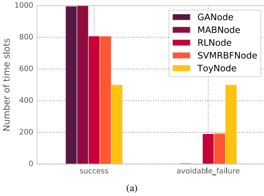
Fig. 12. Choice of the channel: number of time slots used by successful transmissions and failures that could have been avoided by selecting a different channel, (a) for all firmwares and (b) for the best five firmwares of each class.
