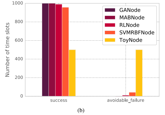
Fig. 12. Choice of the channel: number of time slots used by successful transmissions and failures that could have been avoided by selecting a different channel, (a) for all firmwares and (b) for the best five firmwares of each class.
