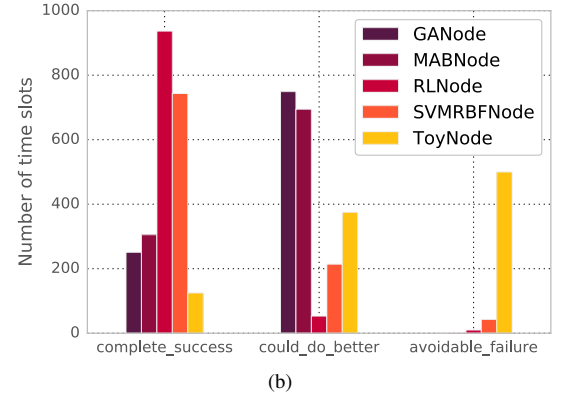
Fig. 11. Choice of the MCS: number of time slots used by entirely successful transmissions, transmissions that could have used a higher performing MCS, and failures that could have been avoided by selecting a different MCS, (a) for all firmwares and (b) for the best five firmwares of each class.
