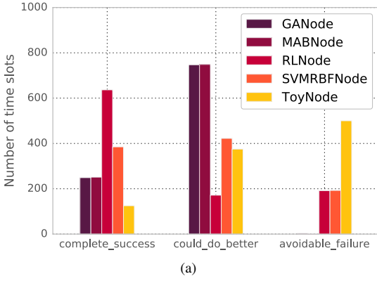
Fig. 11. Choice of the MCS: number of time slots used by entirely successful transmissions, transmissions that could have used a higher performing MCS, and failures that could have been avoided by selecting a different MCS, (a) for all firmwares and (b) for the best five firmwares of each class.
