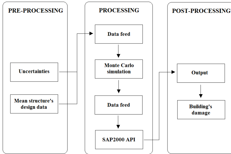
Figure 1. Data flow.
