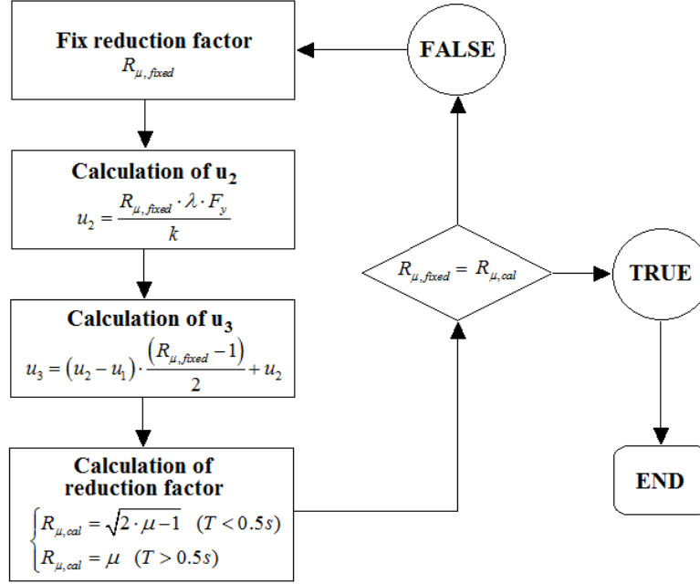
Figure 7. Iterative procedure for evaluating the reduction factor.
