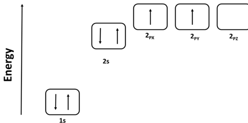
Figure 1.1: Energy levels of carbon atom.
