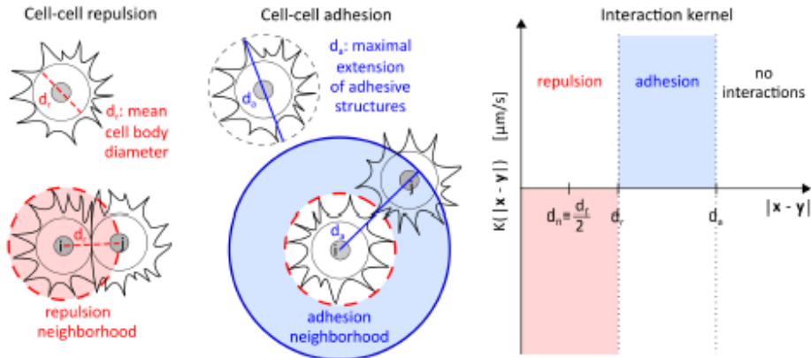
Figure 1: Left panels: Repulsive interactions affect the dynamics of two cells when their relative distance is lower than a mean cell body diameter d_r . The repulsive neighborhood of each cell i , with i = 1, \dots, N , then consists of a round area with radius d_r centered at the actual position of particle i . Central panels: Attractive interactions arise between cells whose relative distance is larger than the mean cell body diameter d_r and lower than the maximal possible extension of cell membrane adhesive structures d_a . The cell adhesive neighborhood then consists of a circular ring with inner radius d_r and external radius d_a . Right panel: The radial interaction kernel K is assumed negative when repulsive, i.e., K(|\mathbf{x} - \mathbf{y}|) < 0 when |\mathbf{x} - \mathbf{y}| < d_r , and positive when attractive, i.e., K(|\mathbf{x} - \mathbf{y}|) > 0 if d_r < |\mathbf{x} - \mathbf{y}| < d_a . Finally, cells whose relative distance is too large do not interact: consistently, we set K(|\mathbf{x} - \mathbf{y}|) = 0 if |\mathbf{x} - \mathbf{y}| > d_a .
