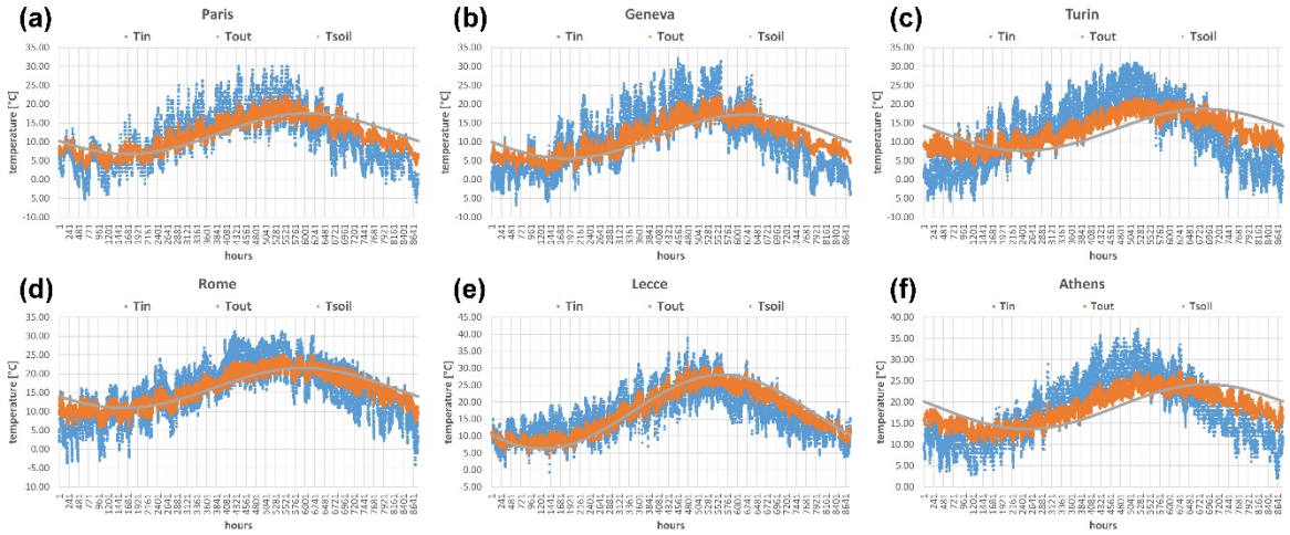
Fig. 2. Yearly variation of the external, ground (3 m depth) and “virtual” EAHX-outlet temperatures for (a) Paris; (b) Geneva; (c) Turin; (d) Rome; (e) Lecce; (f) Athens.
