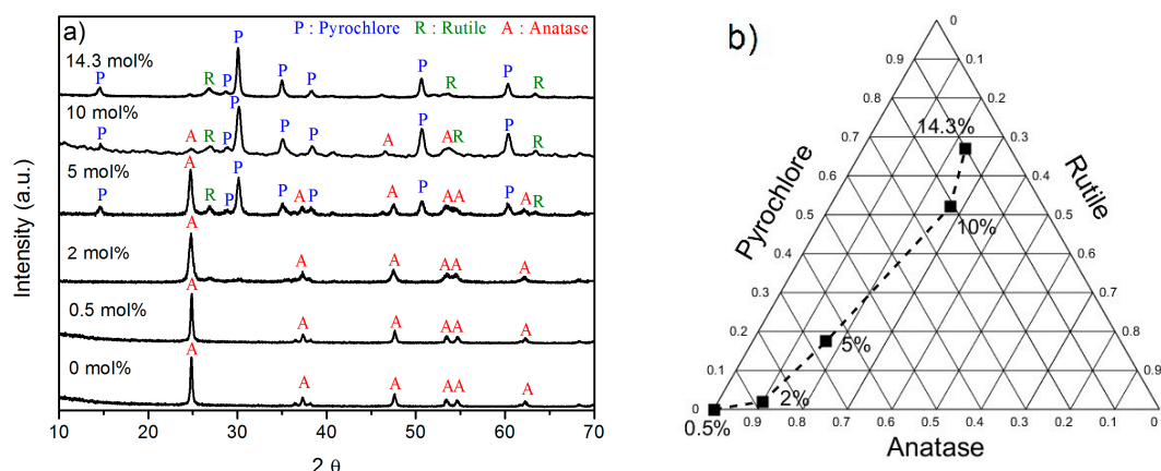
Figure 7. (a) XRD patterns of the undoped and 0.5, 2, 5, 10, and 14.3 mol% \text{Er}_2\text{O}_3 -doped \text{TiO}_2 particles calcined at 800\text{ }^\circ\text{C} for 2 h. The diffraction peaks of the anatase, rutile, and pyrochlore phases are indexed in the figure; (b) Ternary diagram showing the proportion of the crystalline phases present in the 0.5, 2, 5, 10, and 14.3 mol% \text{Er}_2\text{O}_3 -doped \text{TiO}_2 particles calcined at 800\text{ }^\circ\text{C} for 2 h.
