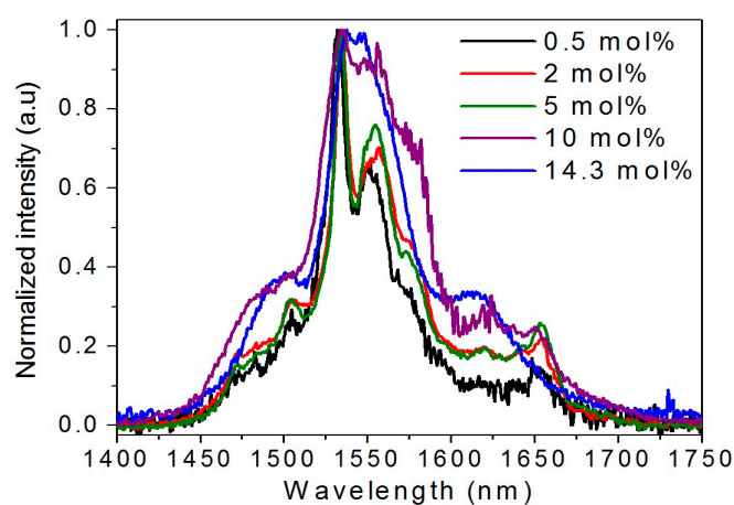
Figure 10. Normalized emission spectra of the 0.5, 2, 5, 10, and 14.3 mol% \text{Er}_2\text{O}_3 -doped \text{TiO}_2 particles calcined at 800\text{ }^\circ\text{C} for 2 h.
