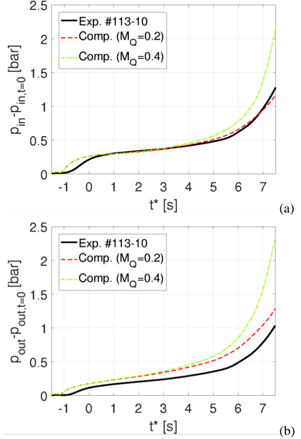
Fig. 33. Comparison between measured (thick solid black) and simulated with two values of M_Q (thin dashed red and thin dash-dotted green, respectively) inlet (a) and outlet (b) pressure. All pressures are rescaled to the respective initial values.
