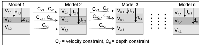
Figure 1. Laterally Constrained Inversion (LCI) scheme: adjacent 1D model are linked by constraints on the model parameters to be resolved (velocity of each layer and interface depths in this example) (modified after Wisen and Christiansen, 2004)
