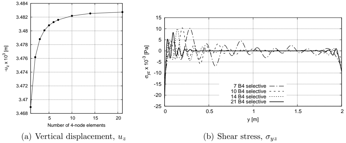
Figure 10: Convergence analysis of the cross-ply beam for an increasing number of 4-node beam elements with selective integration (a) and transverse shear stress distribution at the top face along the beam axis (b) for the four most refined discretizations analyzed in (a).
