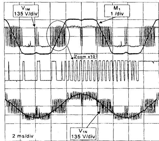
Figure 13 Zone2: \hat{v} = 164/\sqrt{3} V; fac=82Hz; f_{\text{sw}}=5\text{-}20\text{kHz} ;
