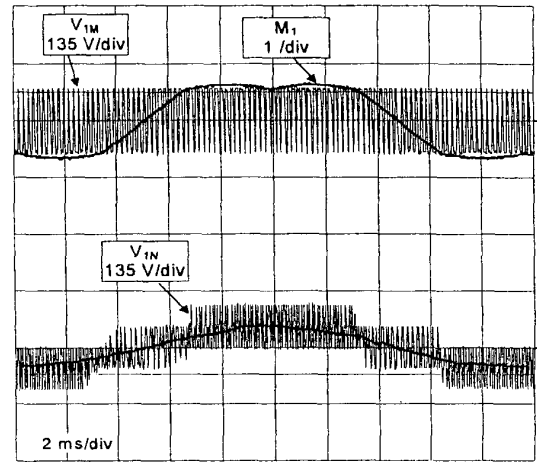
Figure 12 Zone 1: \hat{v} = 100/\sqrt{3} V; fac=50Hz; f_{\text{sw}}=5\text{kHz} ;
