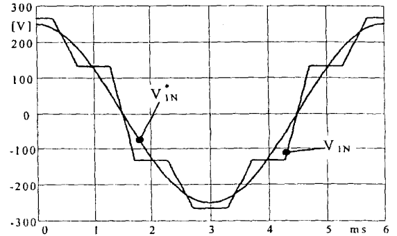
Figure 9: Quasi Six Step mode, @ V=250V , V_C=400V , f_{sw}=166Hz
