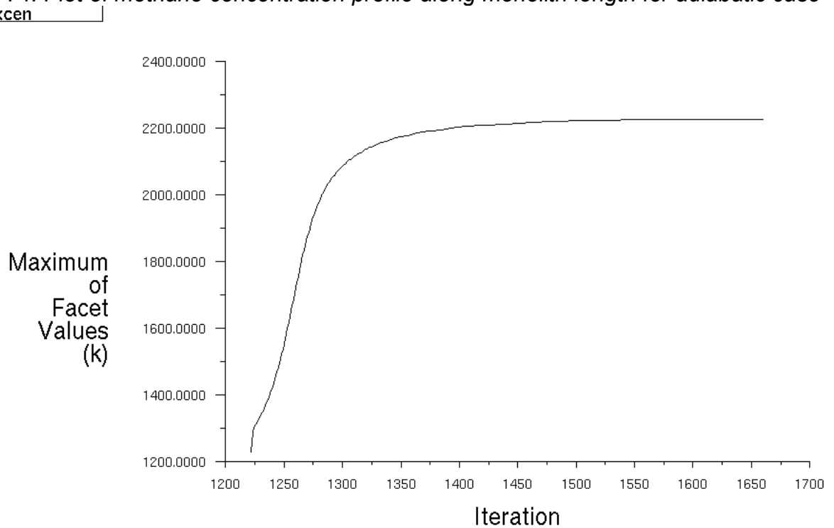
Figure 75: Plot of maximum temperature value at any iteration for adiabatic case.
