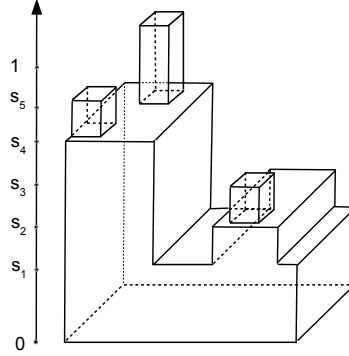
Figure 4: Graph of g with \Sigma(z) not satisfying hypotheses (ii) and (iii)
