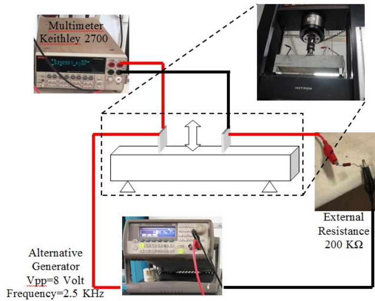
Figure 12- Three-point bending experiment under static and dynamic loading and experiment circuit setup
