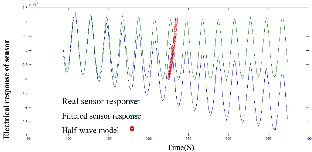
Figure 35- The production of the Half-wave model
