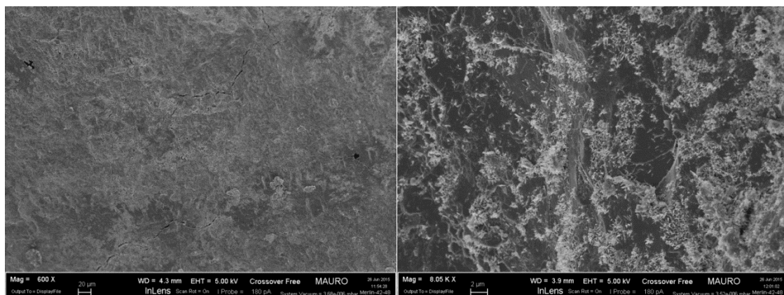
Figure 16- Concrete reinforced with 0.05% wt MWCNTs with SDS as the surfactant and Tributyl Phosphate defoamer.
