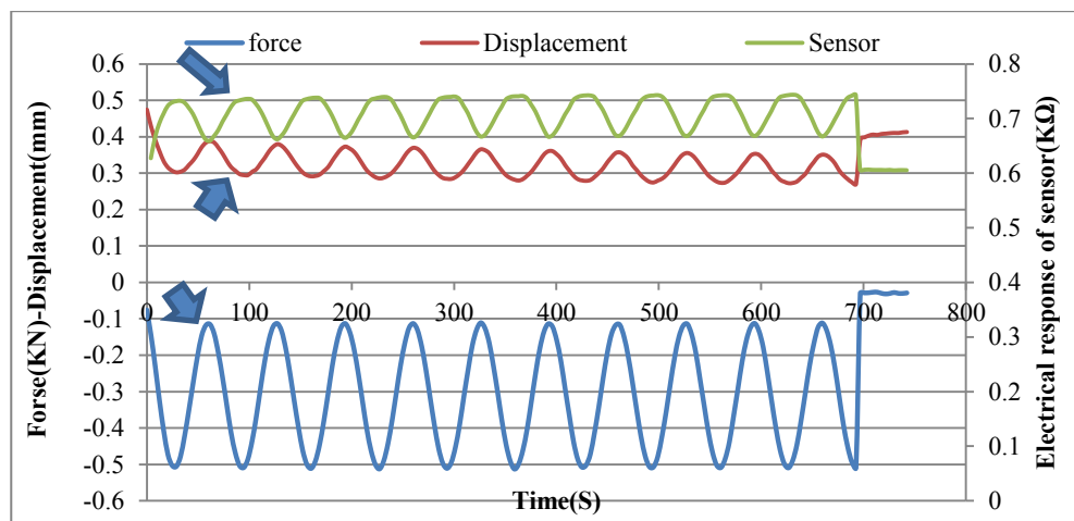
Figure 34- Electrical response of the cement-based sensor, the cement-based sensor movement and applied force against the time
