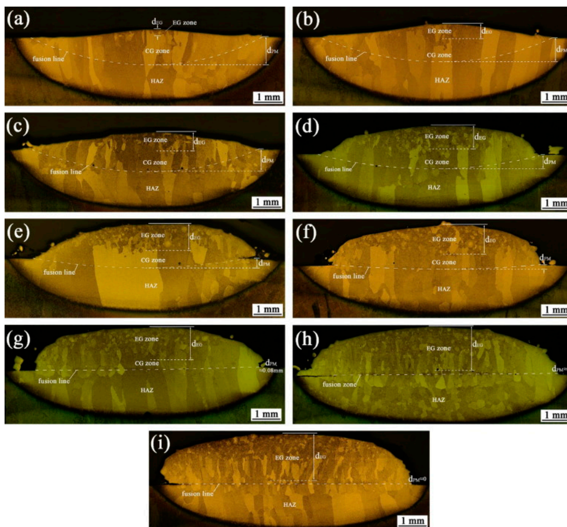
Figure 5. Optical micrographs showing the as-deposited prior beta grain morphologies on transverse cross section of single-track deposited specimens as a function of mass deposition rate, (a) 6 g/min, (b) 11 g/min, (c) 15 g/min, (d) 25 g/min, (e) 31 g/min, (f) 36 g/min, (g) 44 g/min, (h) 55 g/min and (i) 59 g/min (reproduced with permission from [87] Copyright Elsevier, 2015).
