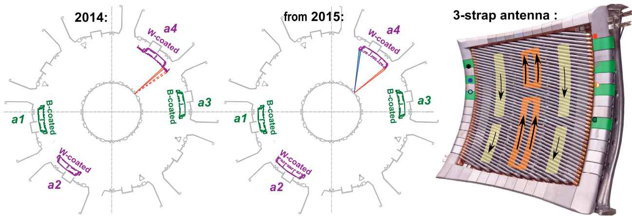
Fig. 1. (Left): 2014 AUG 2-strap antenna configuration. Middle: configuration from 2015 with 3-strap antennas. Right: view of AUG 3-strap antenna a_4 with diagnostics and the RF currents at the surfaces of the straps closest to the plasma.
