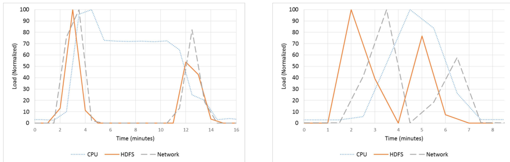
(a) BigFIM: Resource utilization
