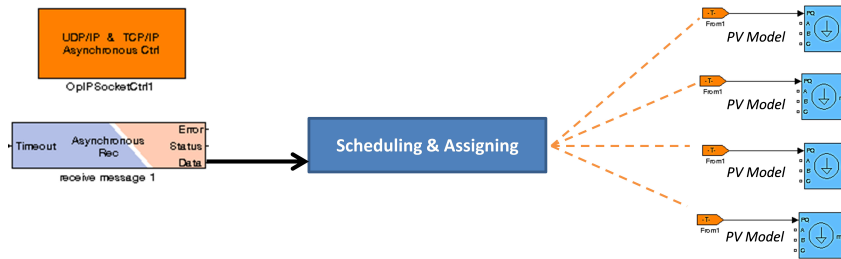
Fig. 3. Real time simulator receiving data links to the distributed PV models over the grid
