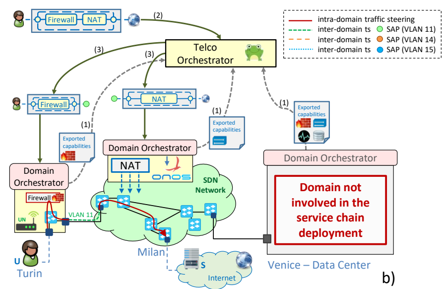
Fig. 4. Validation scenario: (a) service chain split across three domains; (b) service chain deployed in two domains.
