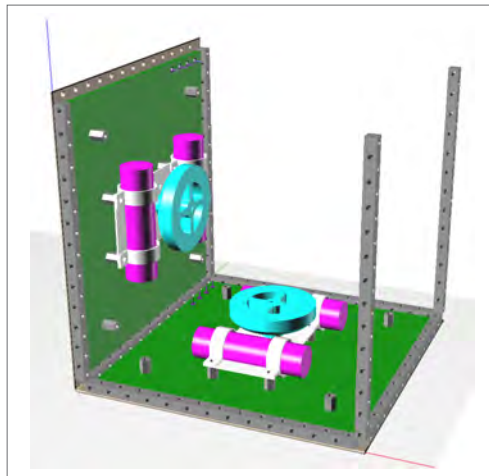
5 Simulation representation of the AraMiS satellite cubic structure, comprehensive of two basic AOCS tiles
