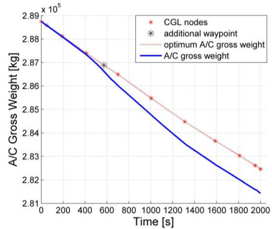
Figure 9. A/C gross mass adopting the FMS#3 and n_{split} = 3 .
