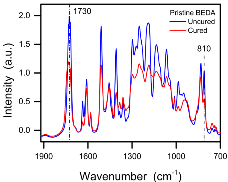
Figure 3. FTIR spectra of pristine BEDA before and after UV curing
