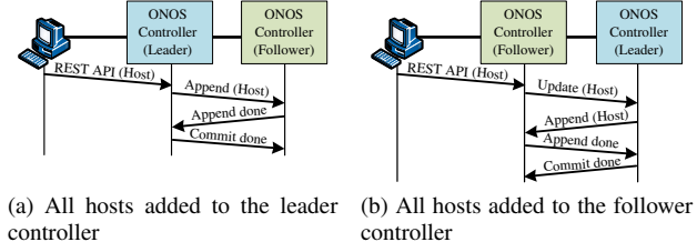
Fig. 18: Scenario with 2 controllers for distributed host store
