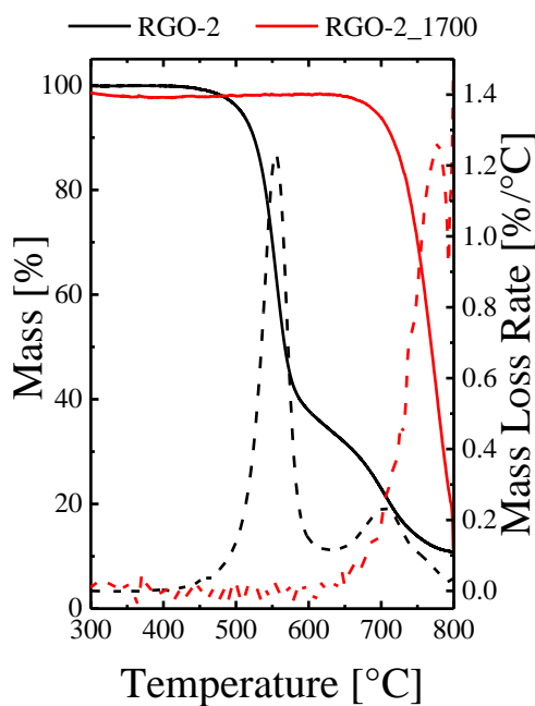
Figure 23. Mass vs. temperature (solid lines) and Mass loss rate vs. temperature (dashed lines) plots for RGO-2 and RGO-2_1700.
