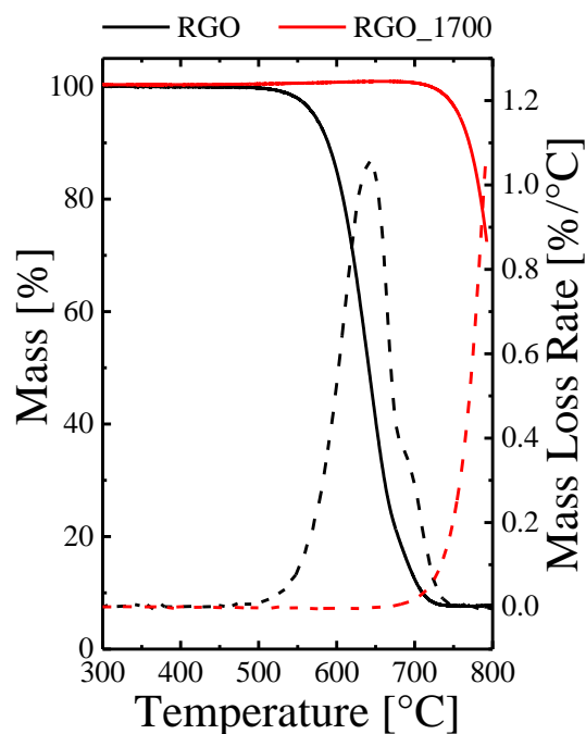
Figure 19. Mass vs. temperature (solid lines) and Mass loss rate vs. temperature (dashed lines) plots for RGO and RGO_1700
