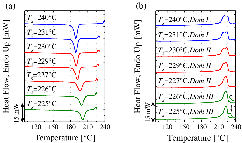
Figure 42. DSC (a) cooling scans from the indicated T_s and (b) heating scans after cooling from the indicated T_s for neat pCBT.
