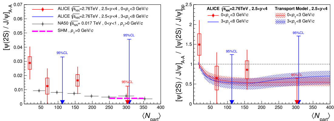
Figure 11. Inclusive [\psi(2S)/J/\psi] ratio measured as a function of \langle N_{\text{part}} \rangle in Pb–Pb collisions at \sqrt{s_{\text{NN}}} = 2.76 TeV for two p_T intervals, compared to NA50 results [29] and to a theoretical calculation [16] (left). Double ratio, as a function of \langle N_{\text{part}} \rangle , between the \psi(2S) and J/\psi measured in Pb–Pb at \sqrt{s_{\text{NN}}} = 2.76 TeV and pp collisions at \sqrt{s} = 7 TeV, compared to theoretical calculations [17] (right).
