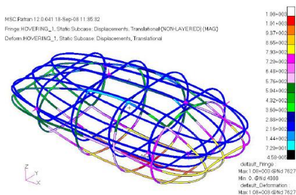
Figure 5 – Exoskeleton of the soap-shaped configuration
