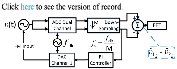
FIG. 2. The scheme proposed allows sampling synchronously one sample per period in order to measure, through its variations, the ADC noise effect on the output, as amplitude and phase fluctuations. The implementation is based on a dual ADC and through the difference of the two outputs the common noise is canceled obtaining only the corresponding noise contribution of each channel.
