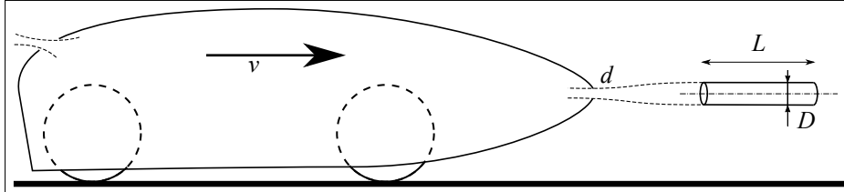
Fig. 2 Schematic representation of the virtual cylinder of air entering the vehicle.
