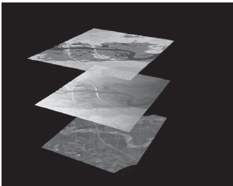
Figure 20.5: Flooding map methodology pertaining to the Orco River. A water surface elevation (middle) is superimposed onto a DTM (below). Subtraction of the two layers allows the water-depths to be obtained.
