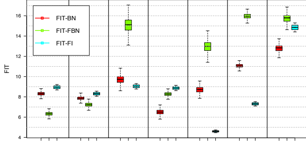
(A) Technology T1 and x86 microprocessor model
