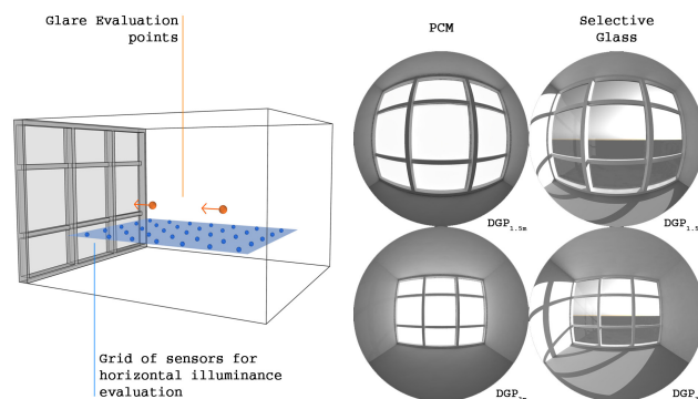
Fig. 1. Left: 3D representation of the sample office model showing the grid of sensors to calculate the E values [blue] and the DGP [orange]. Right: example of images to calculate DGP 1.5m and DGP 3m for the PCM and selective glass.
