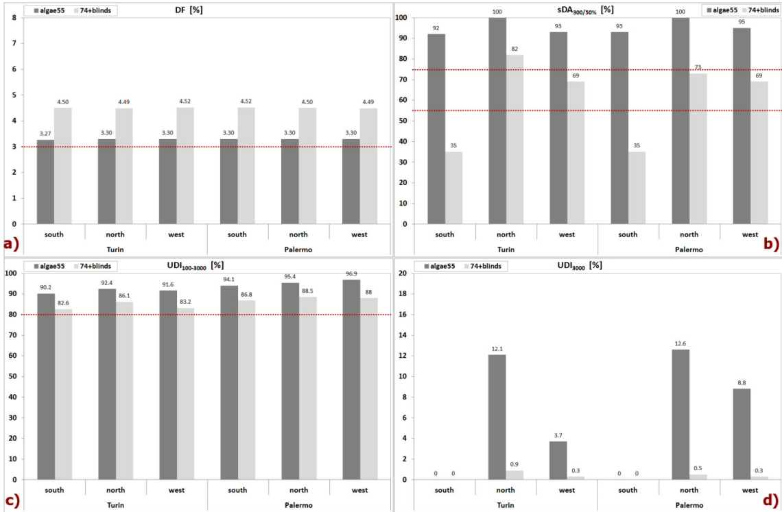
Fig. 5. Comparison of the daylight amount in the same room equipped with the algae-system and with a traditional venetian blind: results in terms of DF (a), sDA_{300/50\%} (b), UDI_{100-3000} (c), UDI_{3000} (d).
