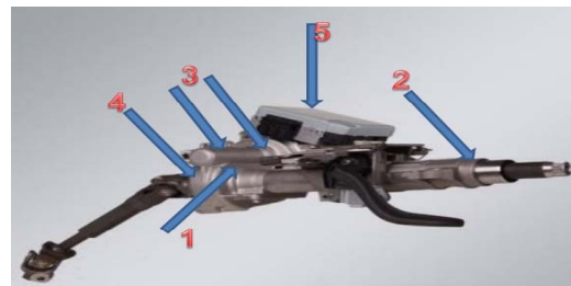
Fig. 1 C-EPS and friction contributions: 1) between worm and gear wheel, 2) between spindle shaft and outer column tube in bearing, 3) in bearings located on the worm shaft, 4) in bearing located on the output shaft, 5) in bearing inside the motor
