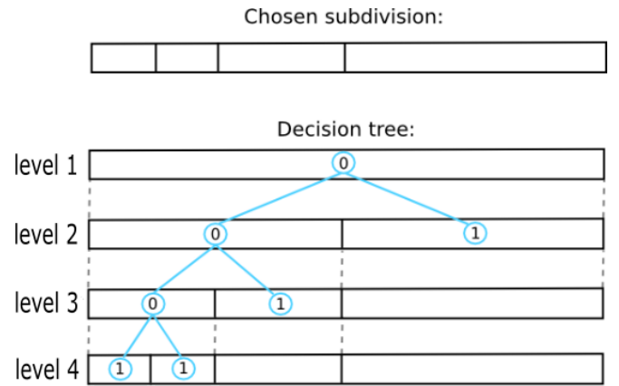
Figure 7. Signaling of the subbands structure: from level 1 downwards, we transmit the labels of the nodes in the binary decision tree.
