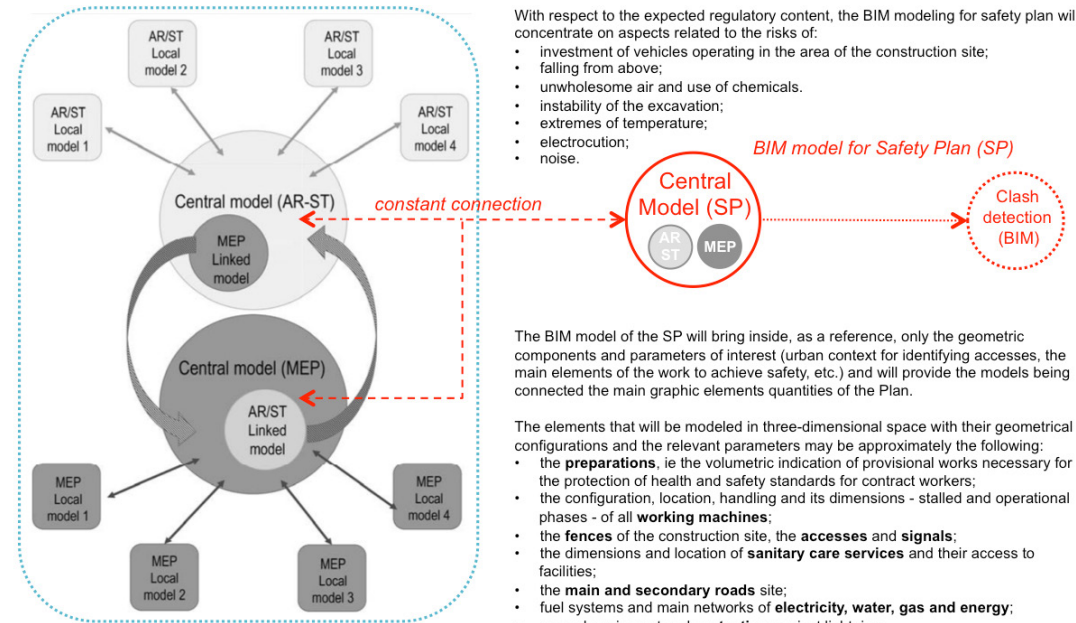
Possible organization of the BIM design environment (with linked models or workset)
