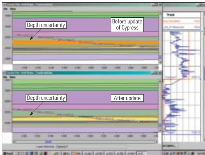
^ Depth uncertainty before and after updating. Before updating ( upper left ), the curtain plot indicates the uncertainty in depth of the Cypress is about 8 feet [2.4 m] (orange band). After the 3D model is updated ( lower left ), the intersection of the well trajectory with the top of the Cypress formation in the model is at a measured depth (MD) of 3020 ft [920 m] (red line), and the depth uncertainty is significantly smaller than before. The vertical axes of the curtain plots ( upper and lower left ) are true vertical depth.
