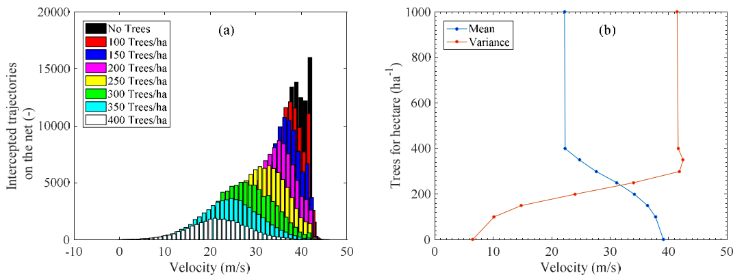
Fig. 2. (a) Distribution of block translational velocity at the collector for different forest scenarios on the slope; (b) variation of mean and variance of the distributions.
