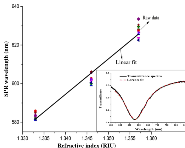
Fig. 5 The resonance wavelength variation with RI; inset shows Lorentz fitting of transmittance spectra.
