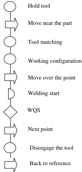
Fig. 2. Workflow of the spot welding manual process
