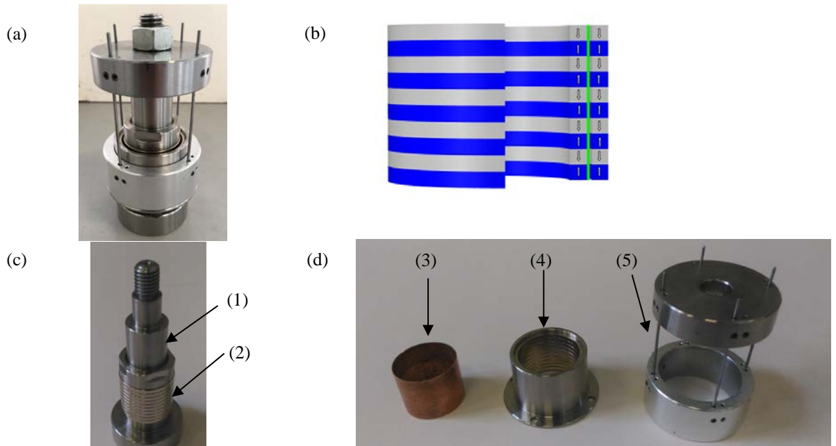
Fig. 6 Test rig used for validation of modeling and identification methods. (a) Complete view, (b) cross –section view of the PMB and ECD, (c), (d) components of the test rig.
