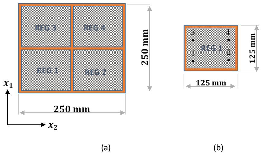
Figure 5.15. Regions indicating Silicon solar cells.
