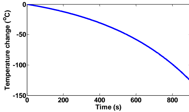
Figure 6.19. Input function for validation of coupled structure preserving model.
