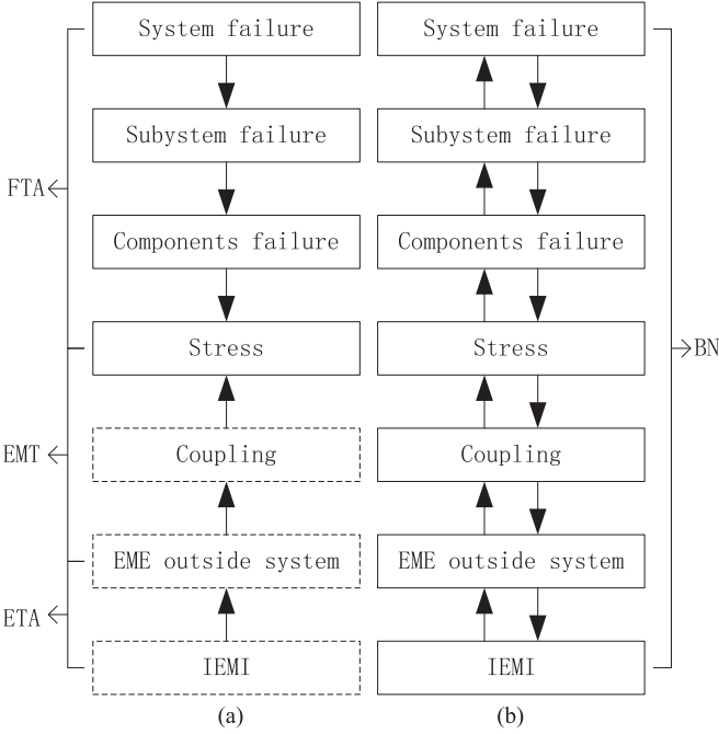
Fig. 5. Comparison of assessment procedures based on FTA and BN. (a) FTA. (b) BN.
