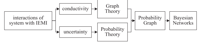
Fig. 1. Derivation of BNs.
