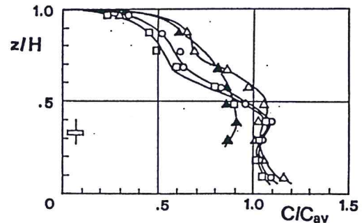
Fig. 1 - Axial concentration profiles at N_j for different types of impeller: \square A310 Lightning; \circ four pitched blade turbine; \Delta six pitched blade disk turbine; \blacktriangledown Rushton turbine. D_p = 100/177 m; B = 0.50 .
