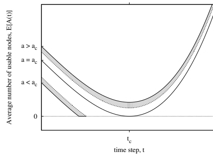
Figure 1: Example of (asymptotic) trajectories of the mean number of usable nodes, \mathbb{E}(A(t)) , with r = 3 . The plot also illustrates by shaded regions the concept of ‘guard zone’.
